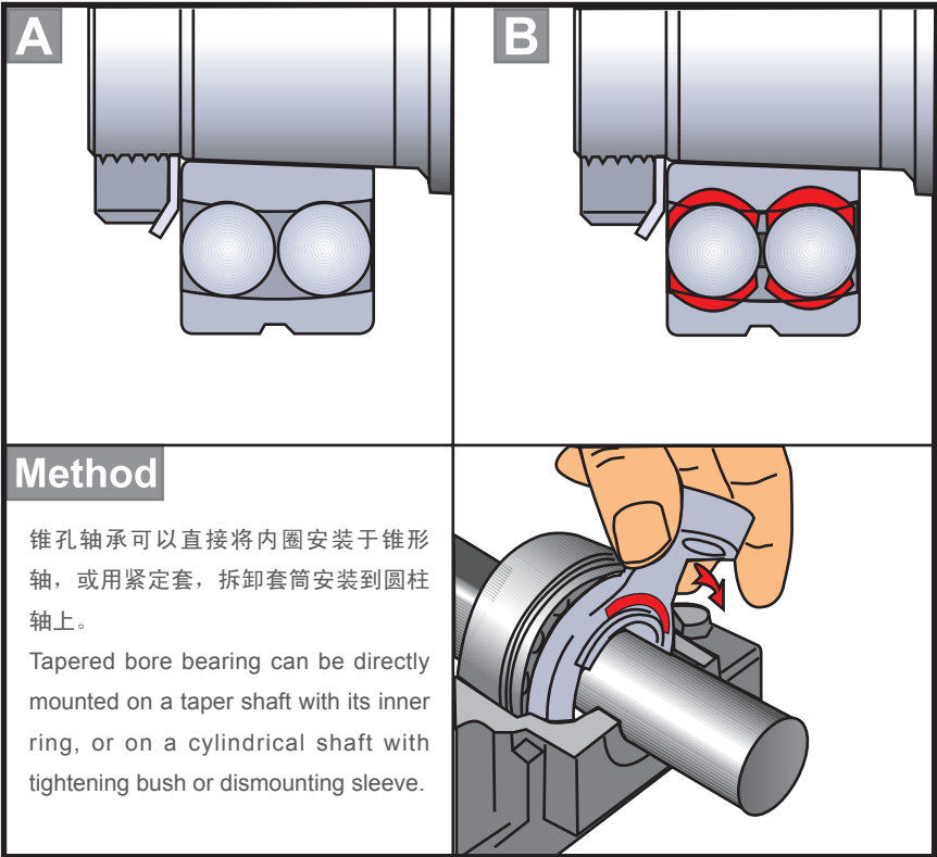
图2.7 锥形孔轴承的安装 Fig.2.7 Tapered bore bearing mounting
